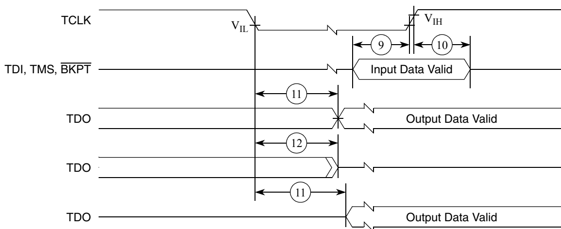
Figure 22. Test Access Port Timing
