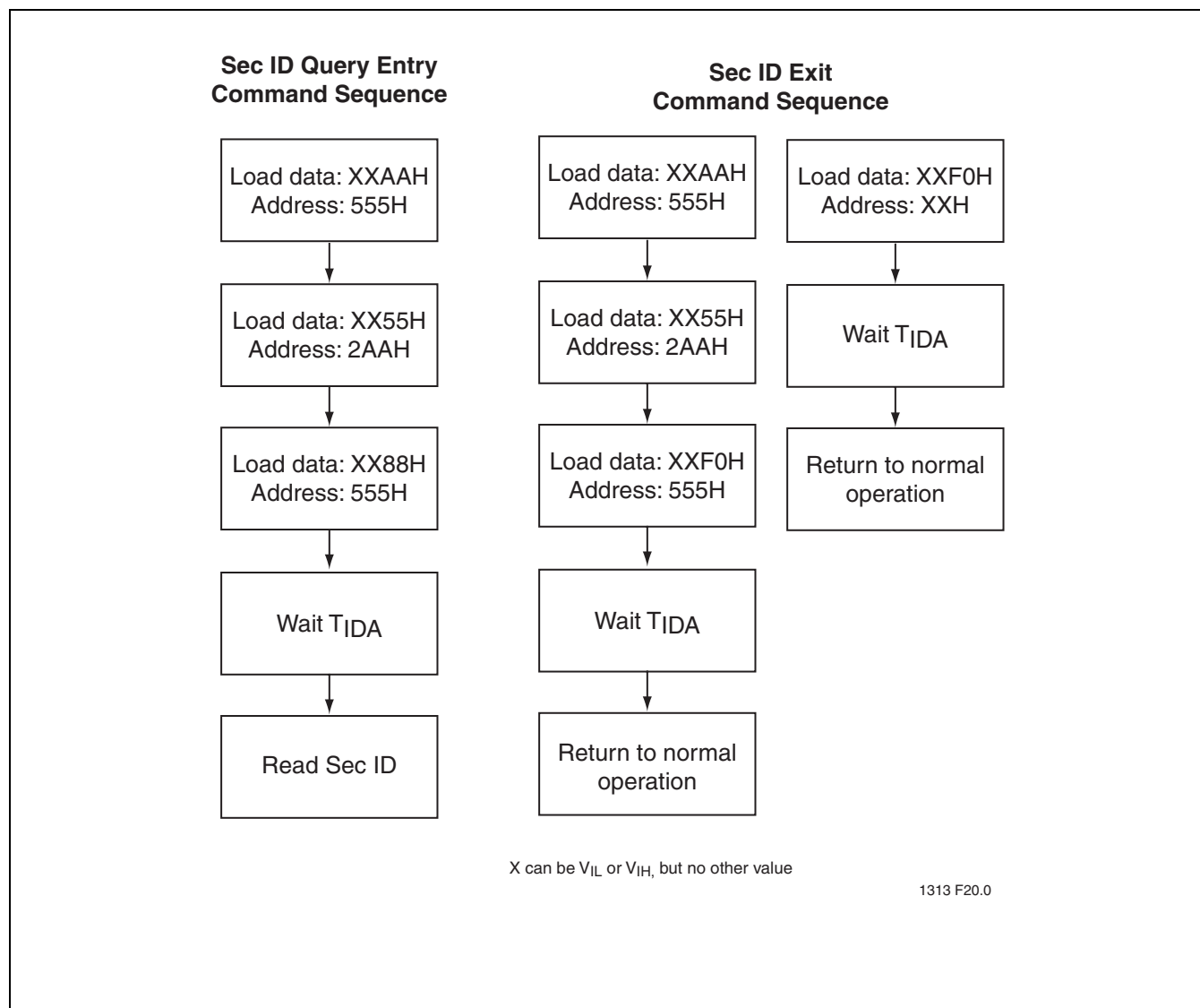
FIGURE 25: Software Sec ID/CFI Command Flowcharts
