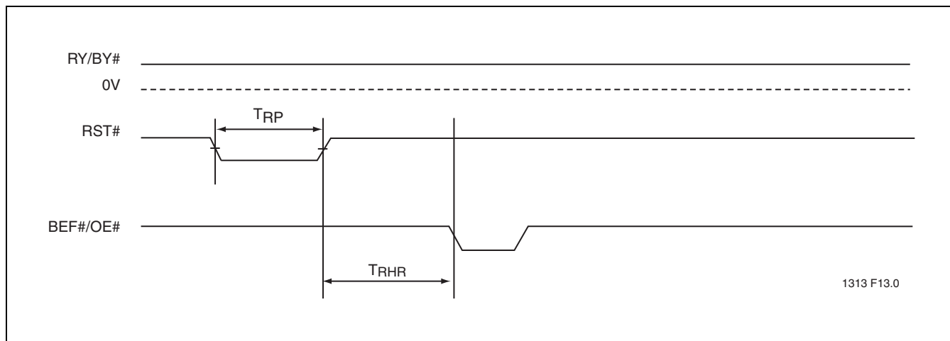
FIGURE 18: RST# Timing (when no internal operation is in progress)
