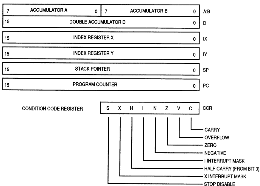
Figure 3–1. Programming Model
