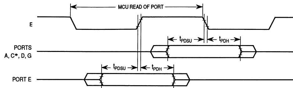
Figure A-8. Port Read Timing Diagram
