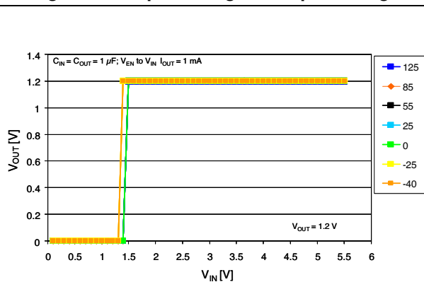
Figure 6. Output voltage vs. input voltage
