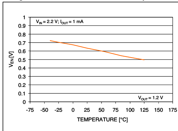
Figure 11. Enable threshold vs. temperature
