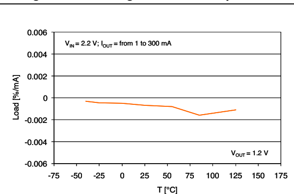
Figure 8. Load regulation vs. temperature
