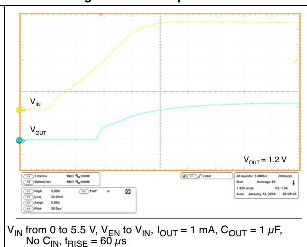
Figure 20. Startup transient
