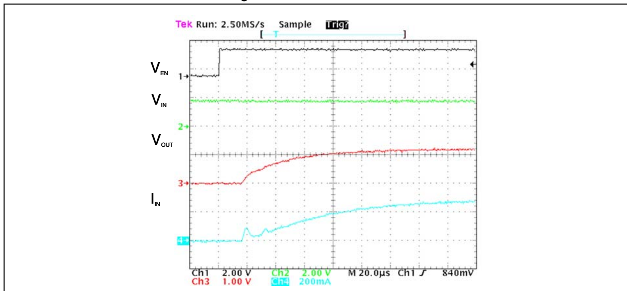
Figure 4. Soft-start function
