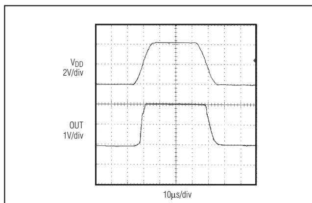
Figure 5. Power-Up/Power-Down Waveform
