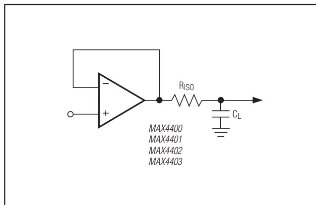
Figure 3. Capacitive-Load-Driving Circuit
