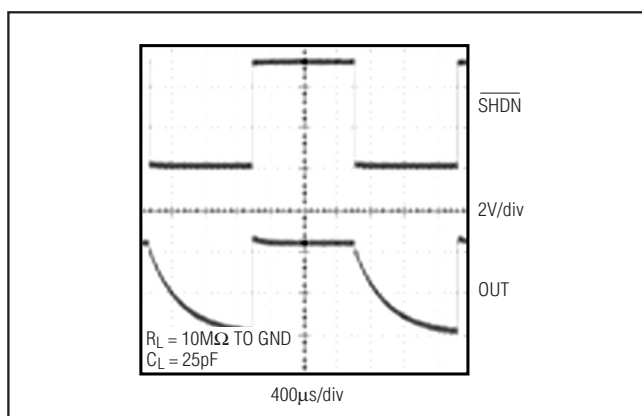
Figure 4. Shutdown Waveform
