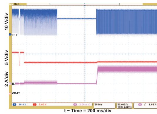
Figure 9. Battery Insertion
