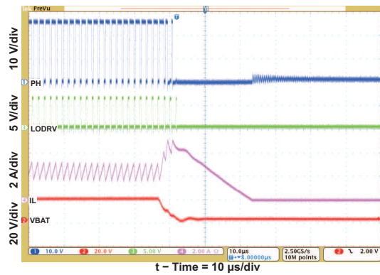
Figure 11. Battery to GND Short Transition
