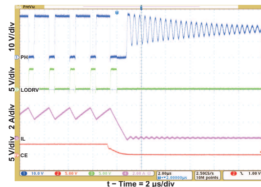
Figure 5. Charge Disable
