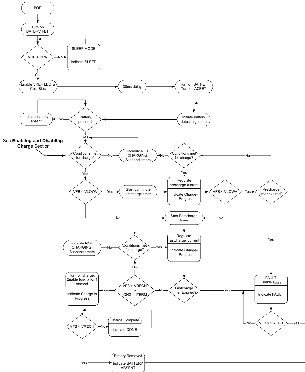
Figure 14. Operational Flowchart
