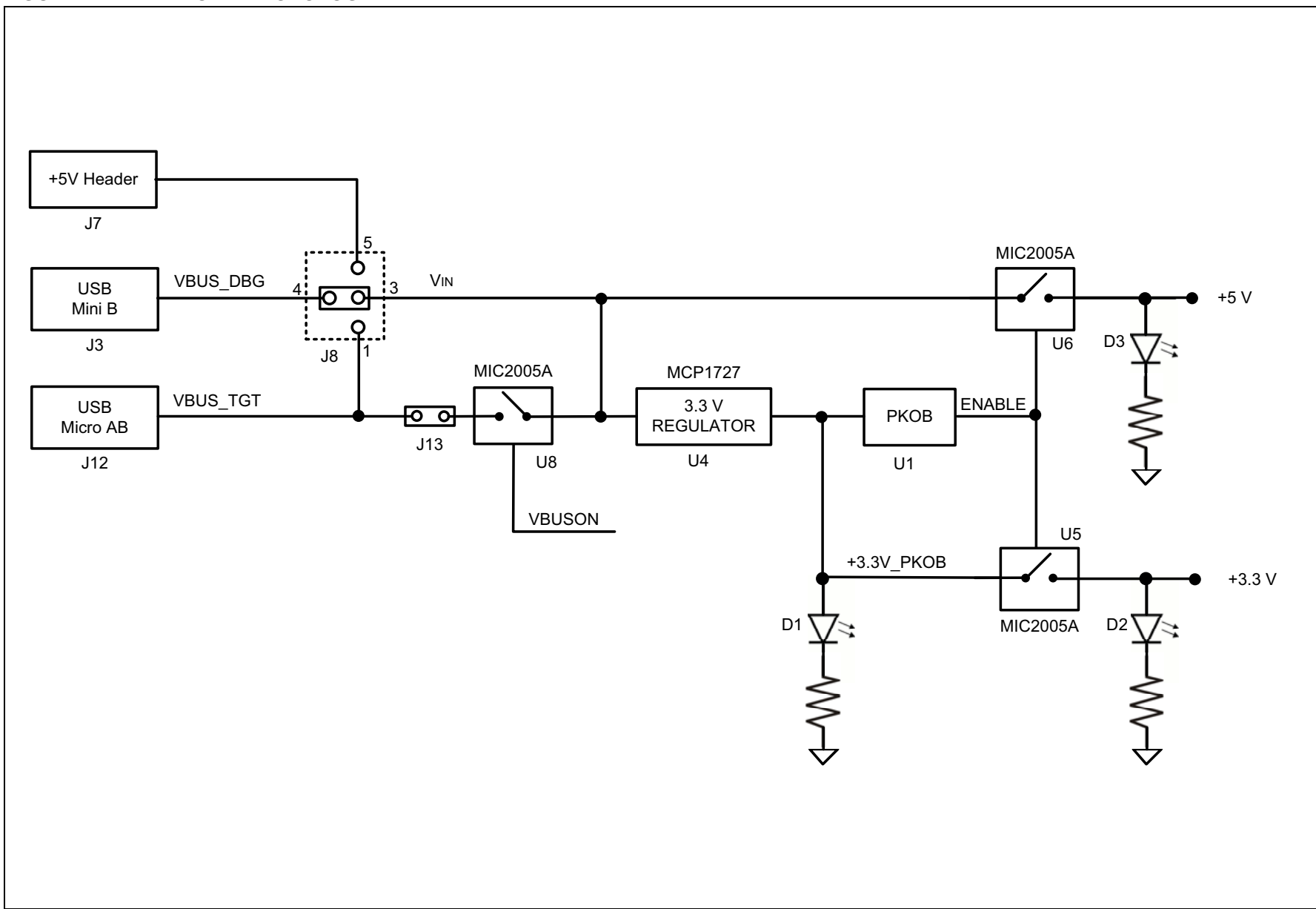
FIGURE 2-1: POWER TOPOLOGY
