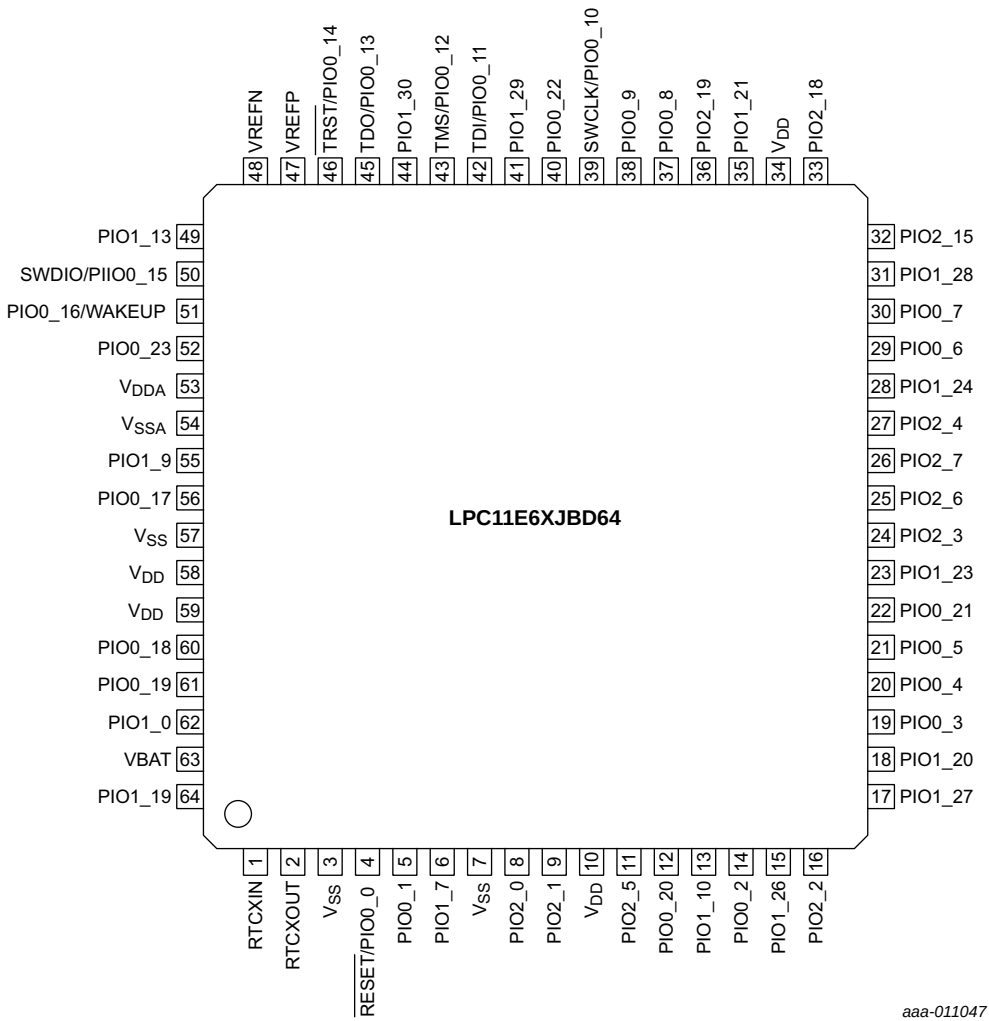
Fig 5. LQFP64 pinning
