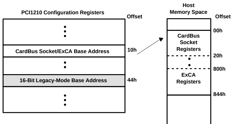
Figure 22. Accessing CardBus Socket Registers Through PCI Memory
