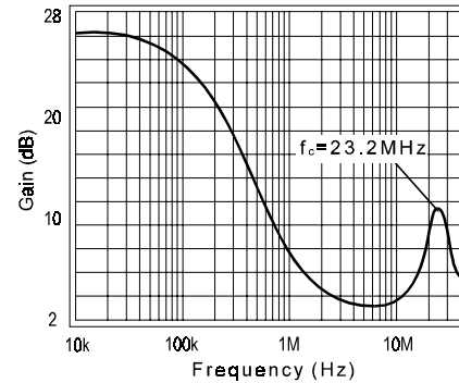
Figure 18: Equalizer Frequency Response
