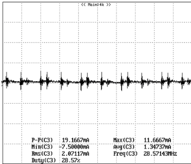
Figure 13: Input reflected ripple current, i_s , through a 12\mu\text{H} source inductor at nominal input voltage and rated load current (20 mA/div, 2 \mu\text{s} /div).
