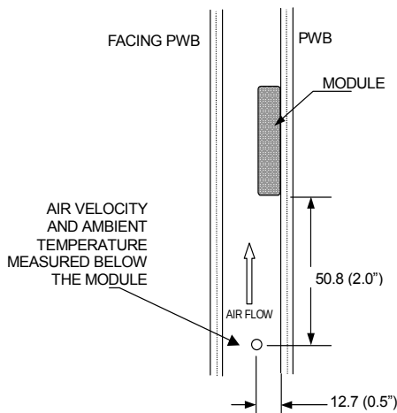
Figure 21: Wind tunnel test setup
