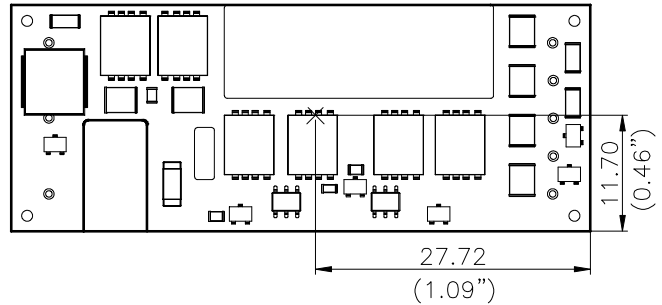
Figure 22: Hot spot location. Pin locations are for reference only. *The allowed maximum hot spot temperature is defined at 123 °C
