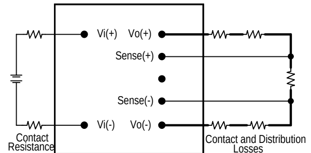
Figure 18: Effective circuit configuration for remote sense operation
