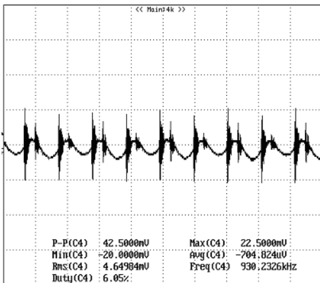
Figure 13: Input reflected ripple current, i_s , through a 12\mu\text{H} source inductor at nominal input voltage and rated load current (20 mA/div, 2 \mu\text{s} /div).
