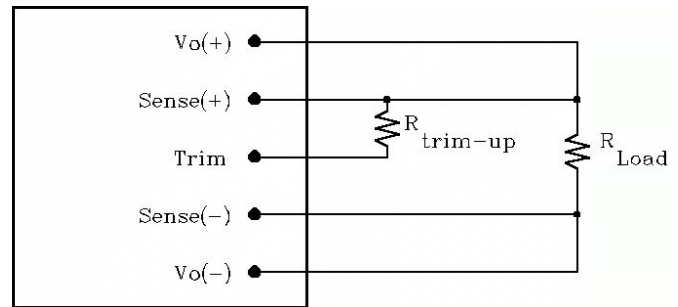
Figure 20: Circuit configuration for trim-up (increase output voltage)
