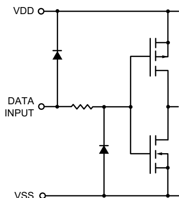
Logic Inputs
