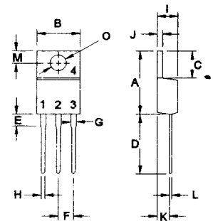
TO-220
