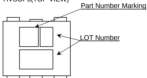
HVSOF5(TOP VIEW)
