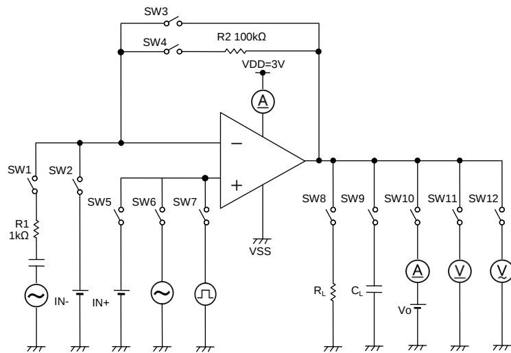
Figure 25. Test Circuit 2
