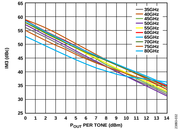
Figure 32. IM3 vs. P_{OUT} per Tone at Various Frequencies at V_{DD} = 4\text{ V} , I_{DQ} = 550\text{ mA}
