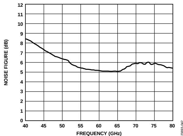
Figure 43. Noise Figure vs. Frequency at 25°C
