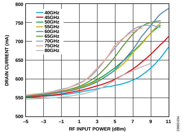
Figure 34. Drain Current vs. RF Input Power at Various Frequencies
