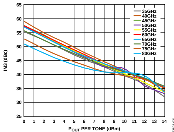
Figure 31. IM3 vs. P_{OUT} per Tone at Various Frequencies at V_{DD} = 3.5\text{ V} , I_{DQ} = 550\text{ mA}
