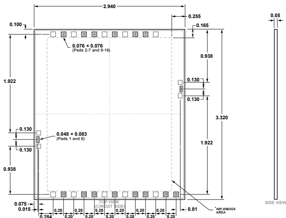
Figure 51. 16-Pad Bare Die [CHIP] (C-16-4)
