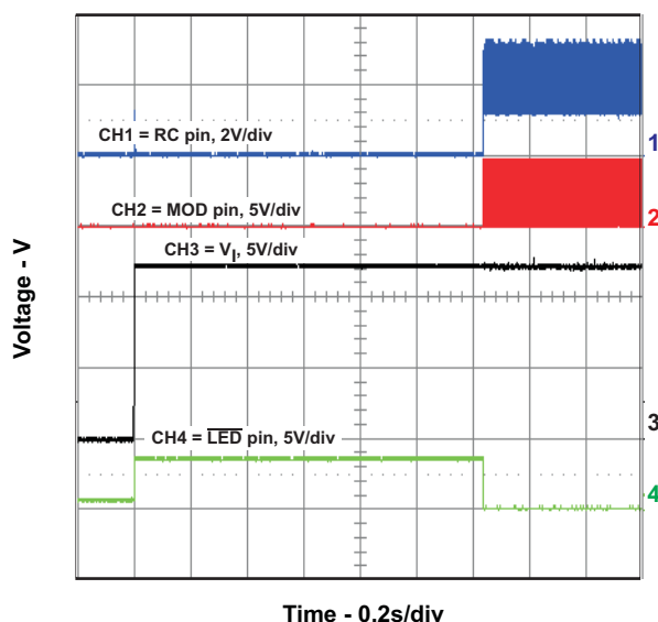
Figure 13. bq2000T Start-up on Vin
