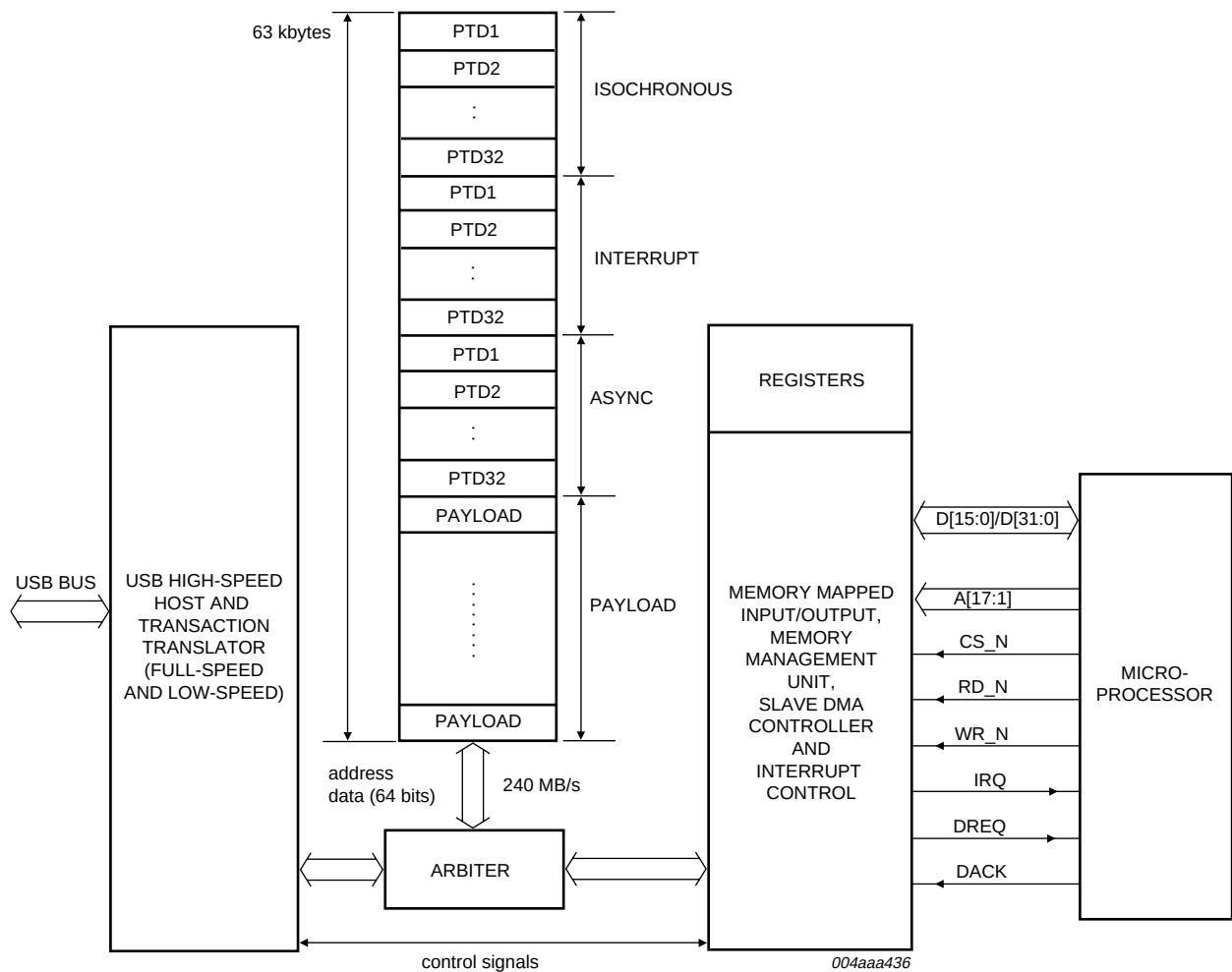
Fig 4. Memory segmentation and access block diagram.
