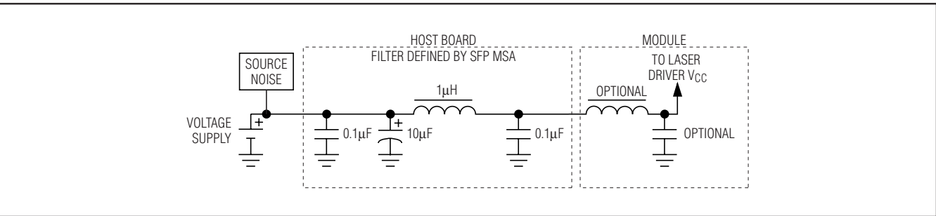
Figure 3. Supply Filter
