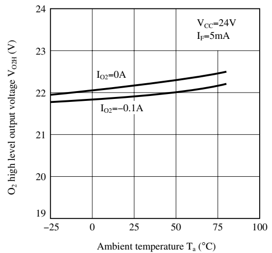
Fig.24 O 2 High Level Output Voltage vs. Ambient Temperature
