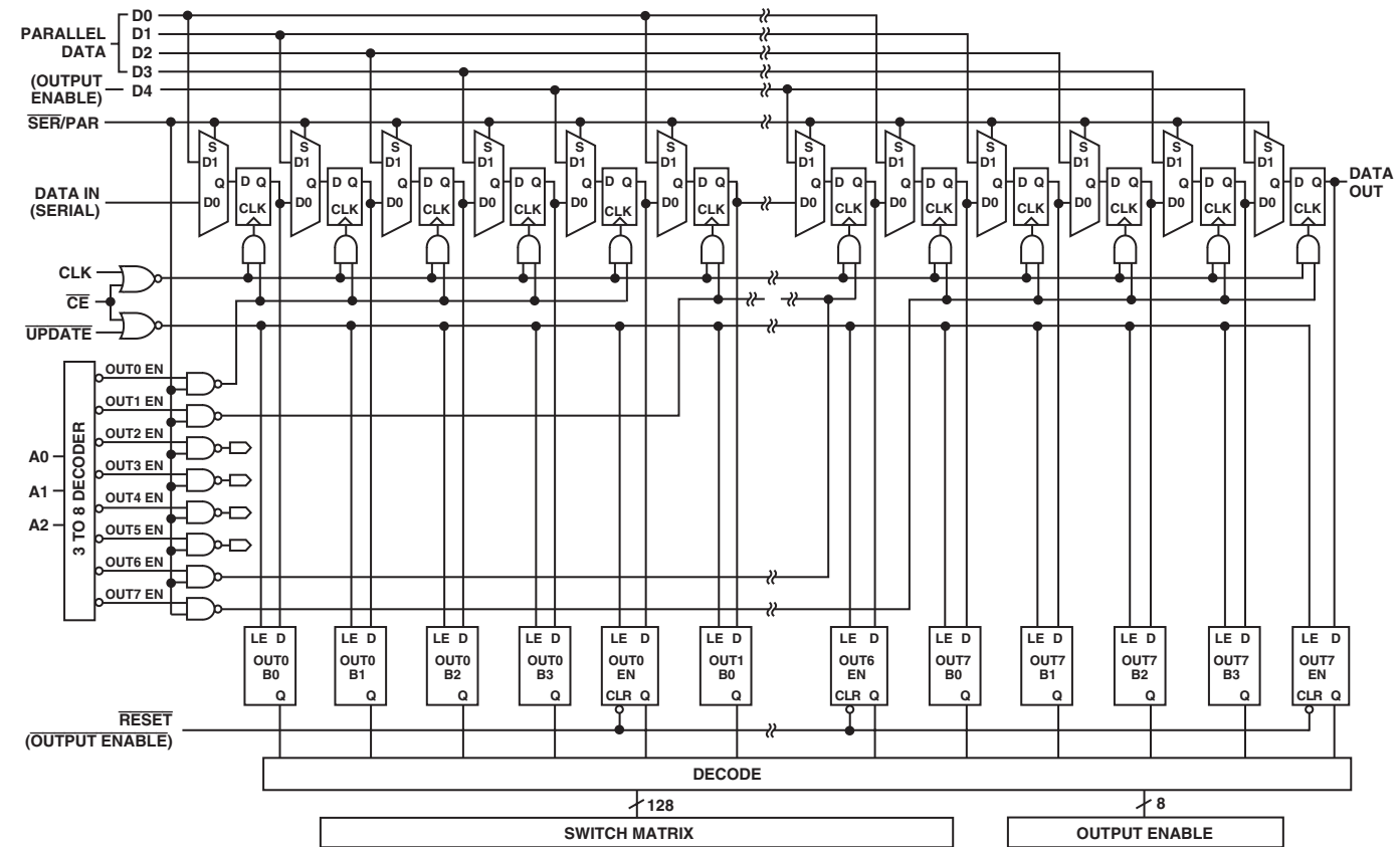
Figure 4. Logic Diagram
