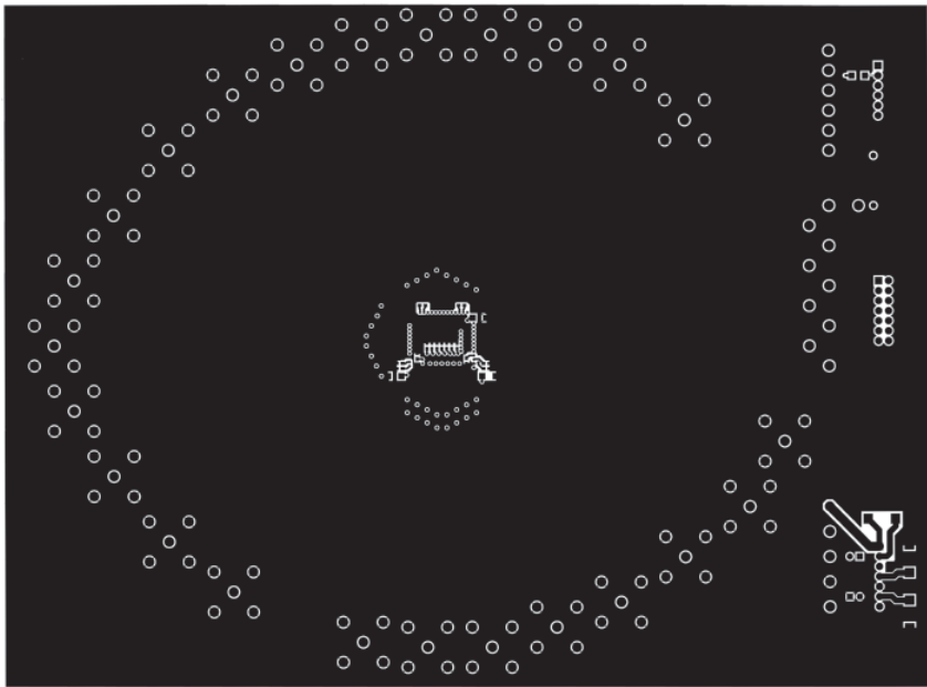
Figure 14. Board Layout (Bottom Layer)
