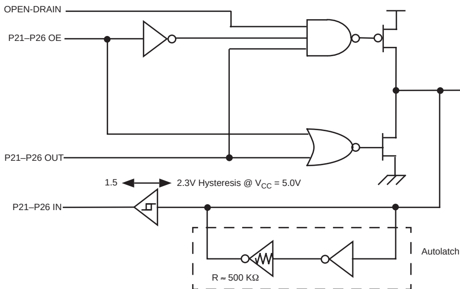
Figure 39. Port 2 Configuration with Open-Drain Capability, Autolatch, and Schmitt-Trigger
