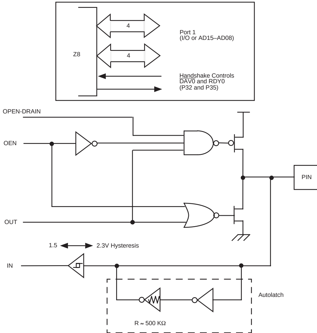
Figure 30. Port 0 Configuration with Open-Drive Capability, Autolatch, and Schmitt-Trigger
