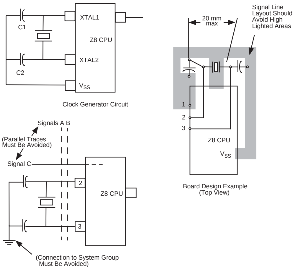
Figure 17. Circuit Board Design Rules
