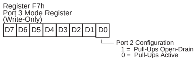
Figure 61. Port 2 Configuration
