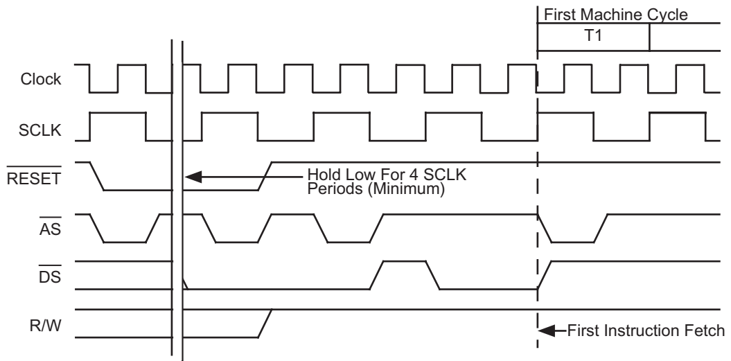
Figure 22. Reset Timing
