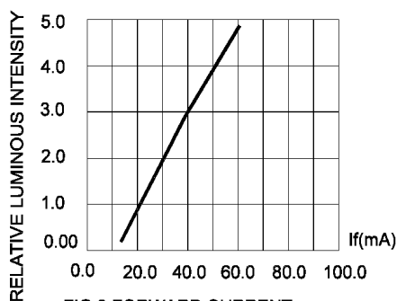
FIG.3 FORWARD CURRENT.
