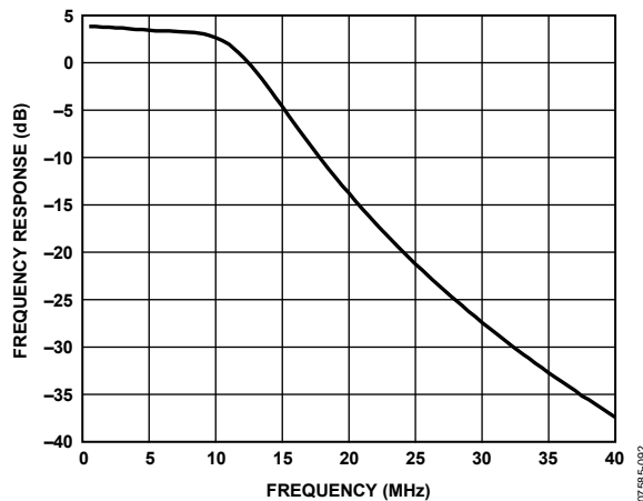
Figure 93. Fourth-Order Low-Pass LTE Filter Magnitude Response
