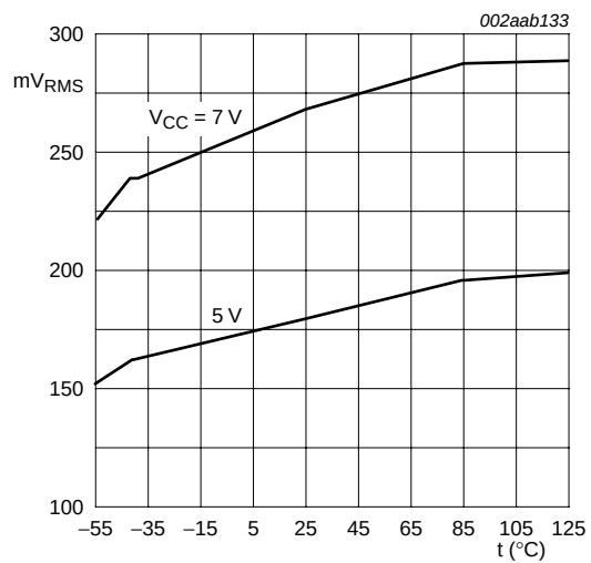
Fig 9. Audio output vs. temperature and supply voltage
