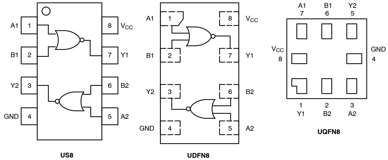
Figure 2. Pinout
