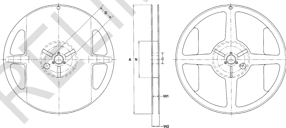
Figure 6 - Reel drawing
