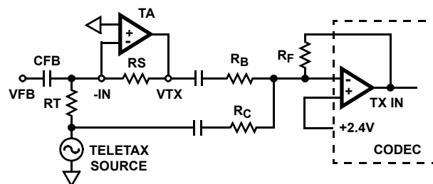
FIGURE 18. TELETAX SIGNALLING
