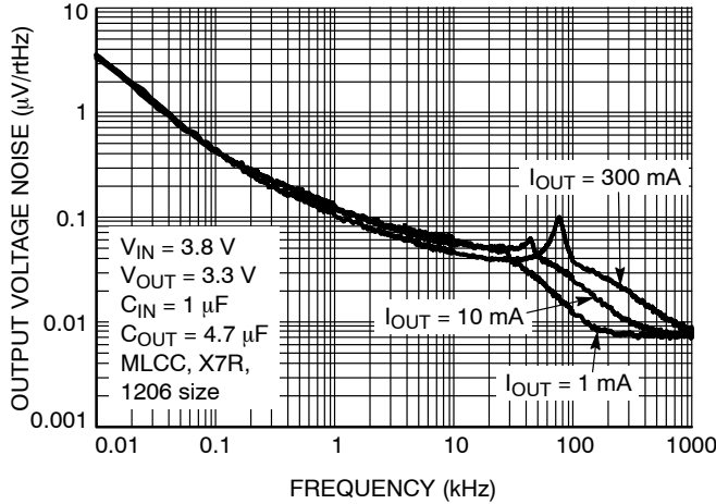
Figure 6. Output Voltage Noise Spectral Density for V_{OUT} = 3.3\text{ V} , C_{OUT} = 4.7\text{ }\mu\text{F}
