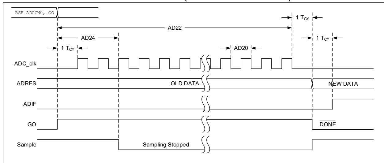
FIGURE 45-10: ADC CONVERSION TIMING (ADC CLOCK F osc -BASED)
