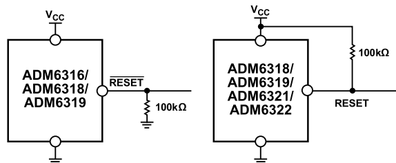
Figure 18. Ensuring Reset Valid to V_{CC} = 0\text{ V}
