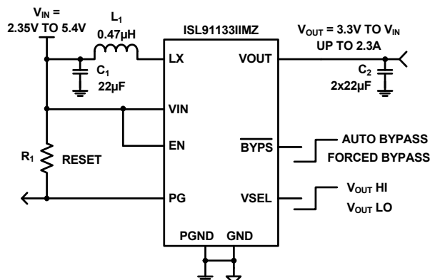
FIGURE 1. TYPICAL APPLICATION
