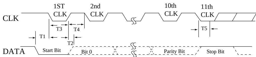
Fig 3. Keyboard output data timings
