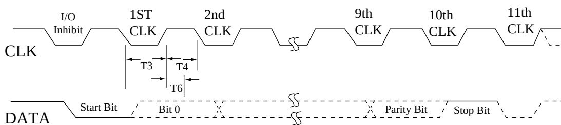
Fig 4. Keyboard input data timings
