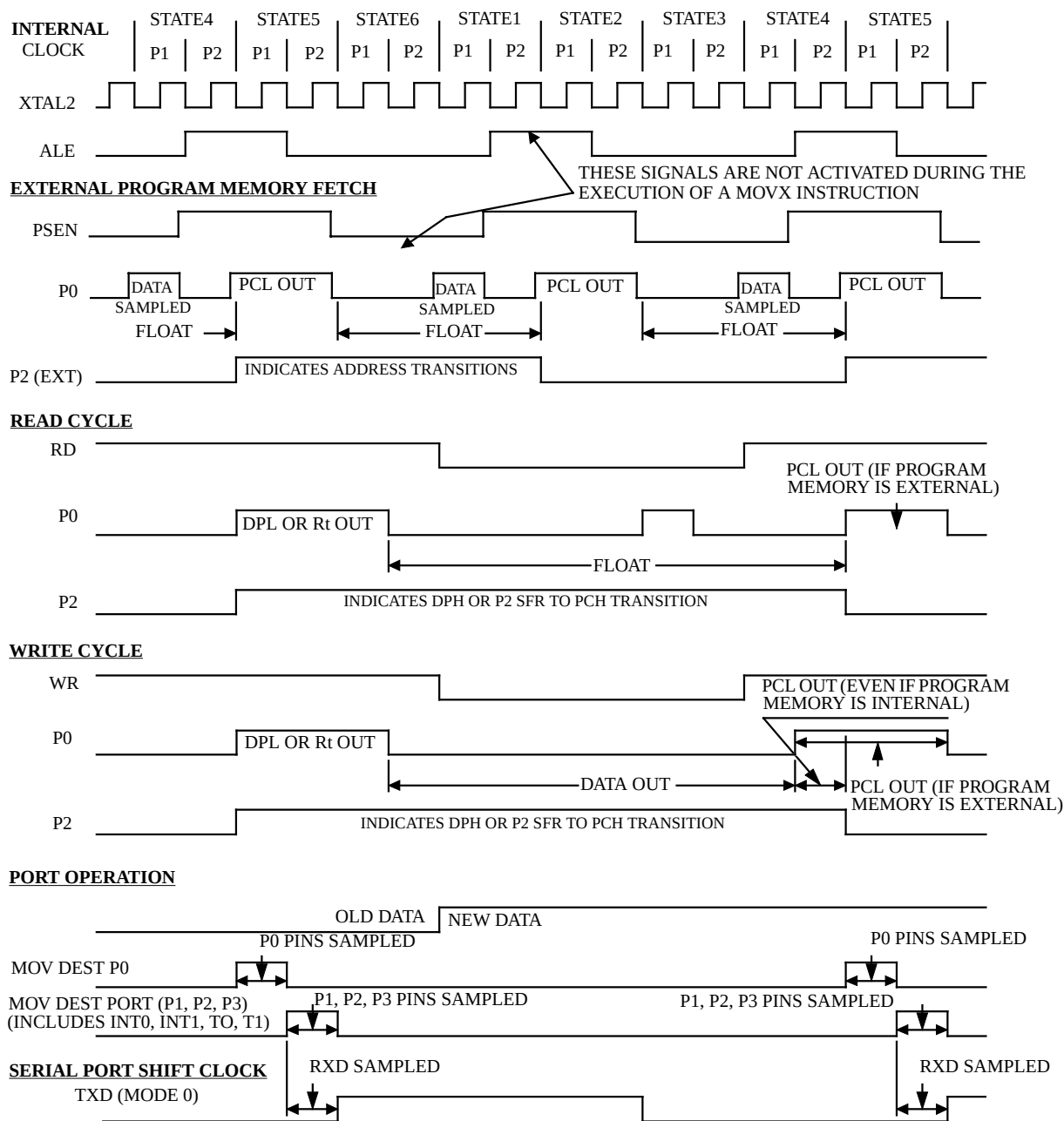
Figure 48. Clock Waveforms
