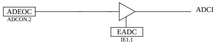
Figure 31. ADC interrupt structure
