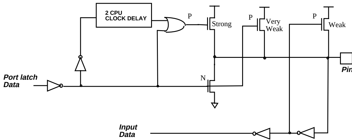
Figure 5. Quasi-Bidirectional Output
