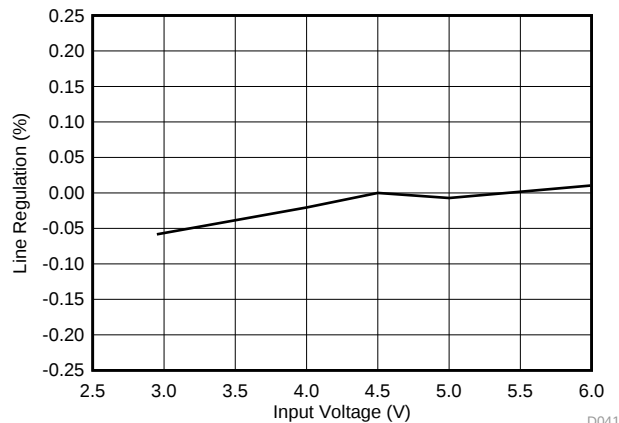
图 51. V_{DD} Output Line Regulation, I_{OUT} = 2 A
