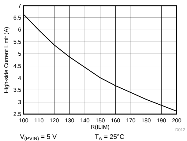
图 12. High-side Current Limit vs R_{\text{ILIM}}
