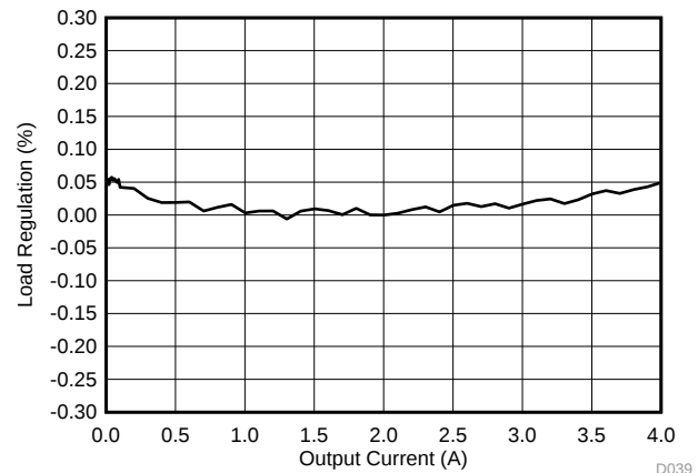
图 50. V_{DD} Output Load Regulation, V_{IN} = 5 V
