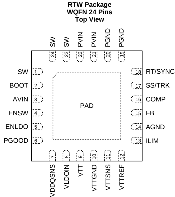
Pin Functions
