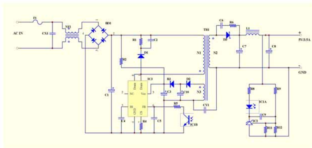
FIG.8 UPS612 Typical Application Circuit
