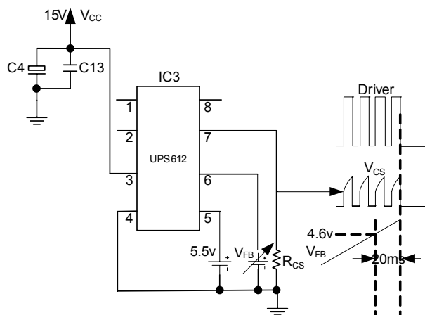
FIG.6 OLP test circuit
