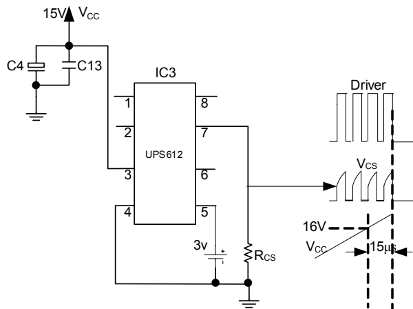
FIG.7 OVP test circuit
