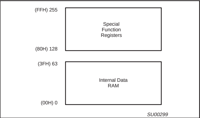
Figure 3. Memory Map
