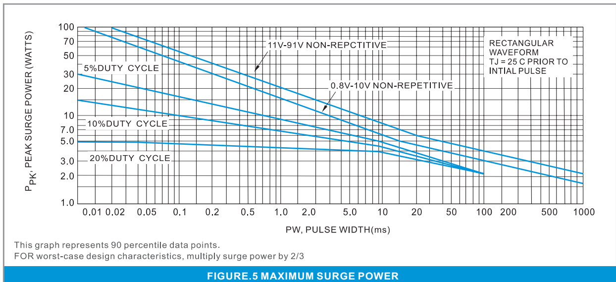
FIGURE.5 MAXIMUM SURGE POWER
