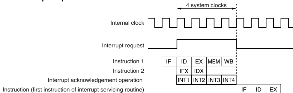
Figure 19-14. Pipeline Operation During Interrupt Request Acknowledgment (Outline)
