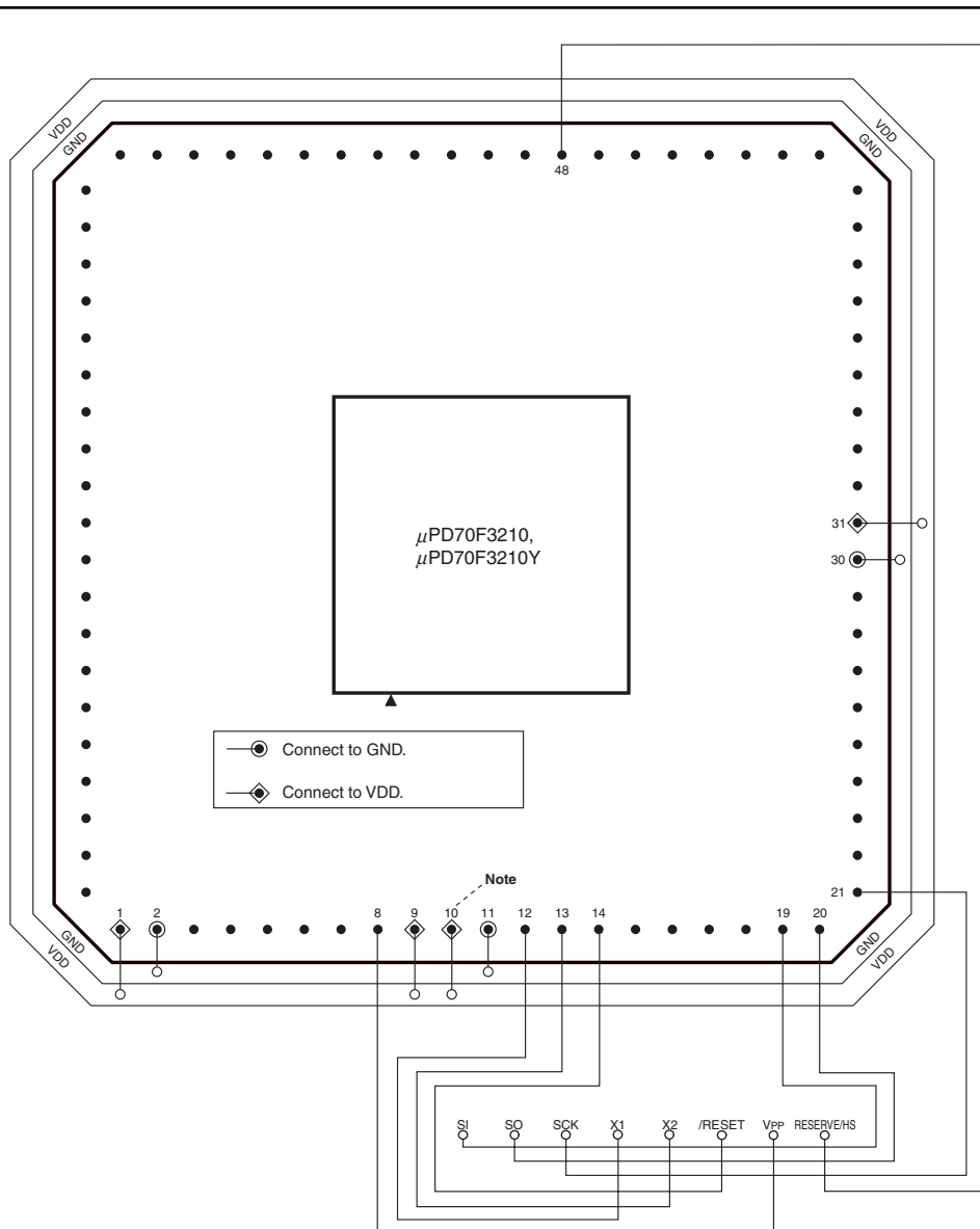
★ Figure 25-1. Wiring Example of V850ES/KF1 Flash Writing Adapter (FA-80GC-8BT, FA-80GK-9EU)
