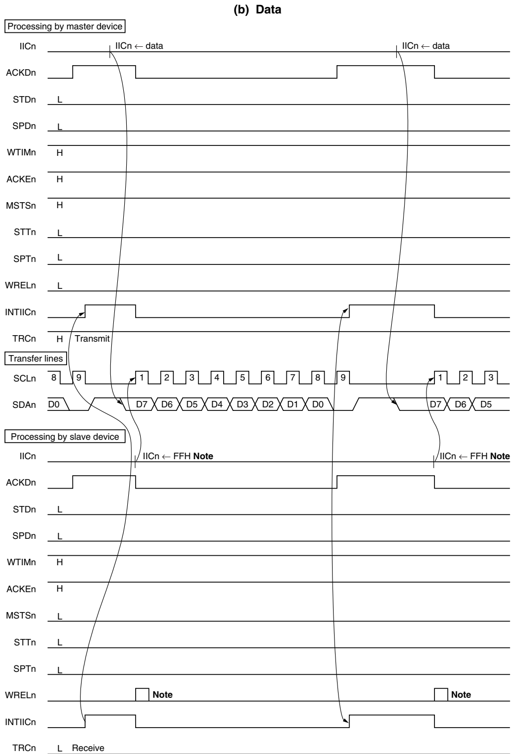
Figure 18-19. Example of Master to Slave Communication (When 9-Clock Wait Is Selected for Both Master and Slave) (2/3)
