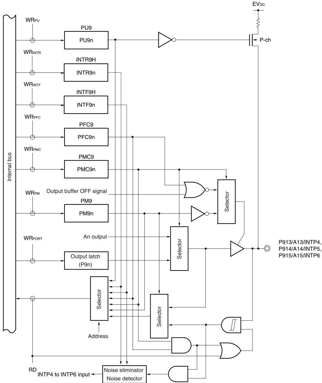
Figure 4-30. Block Diagram of P913 to P915
