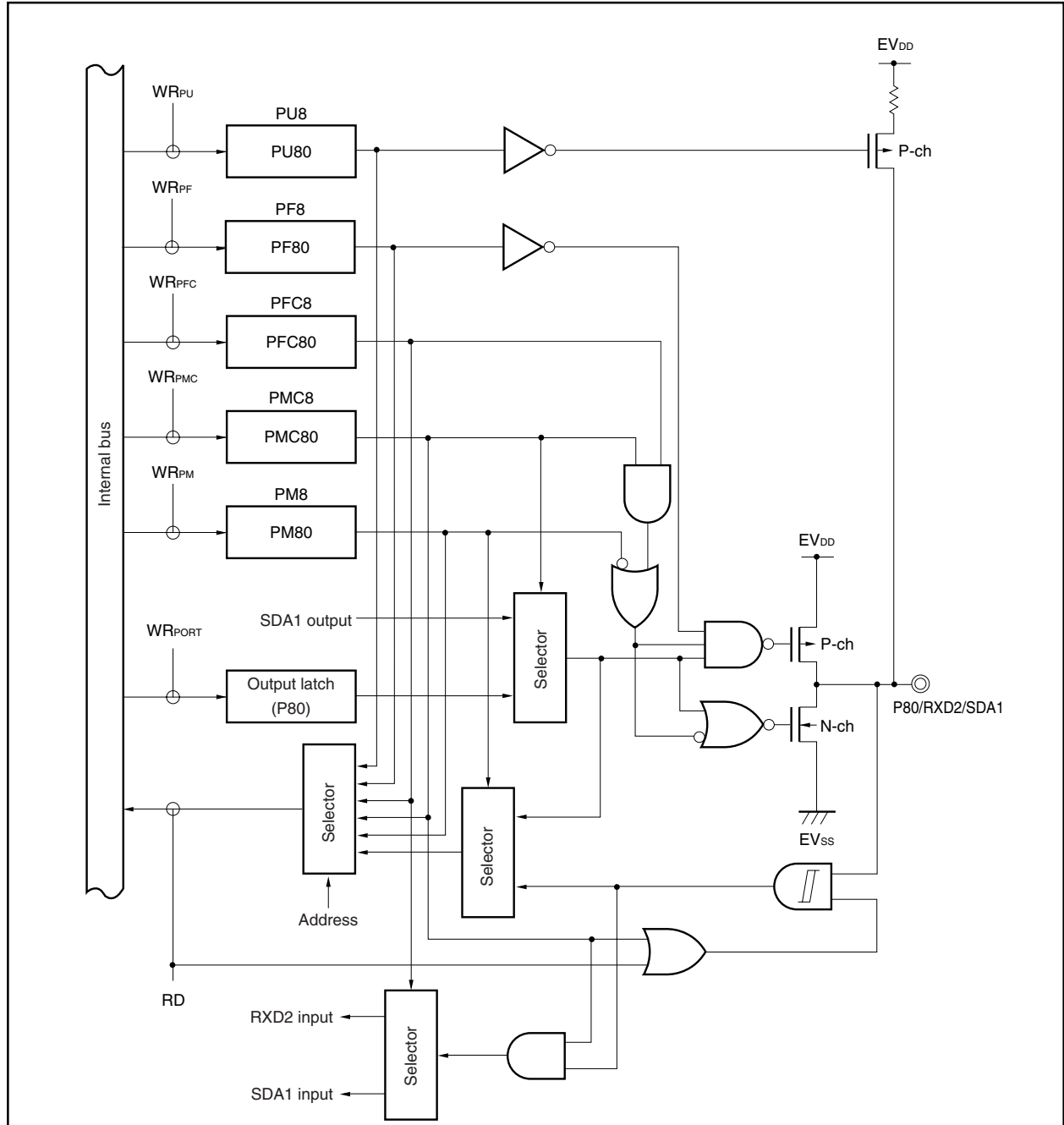
Figure 4-23. Block Diagram of P80
