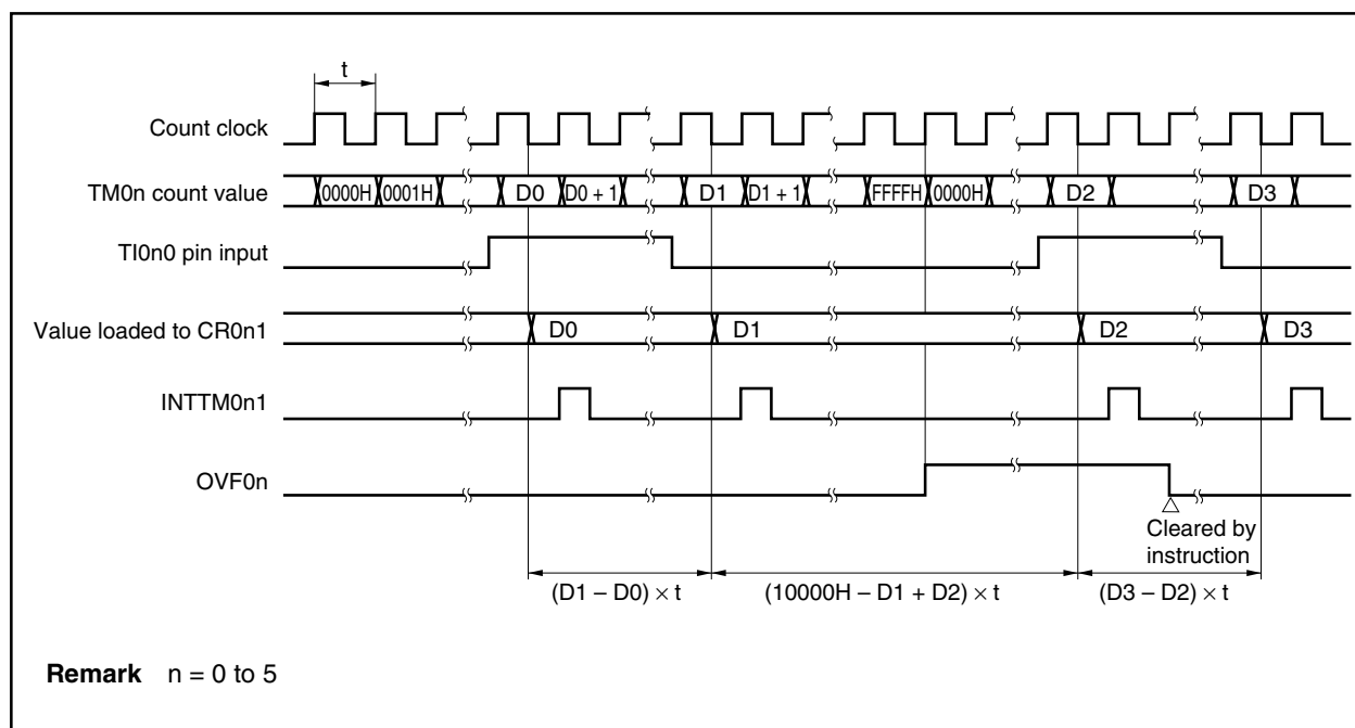
Figure 7-10. Timing of Pulse Width Measurement with Free-Running Counter and One Capture Register (with Both Edges Specified)
