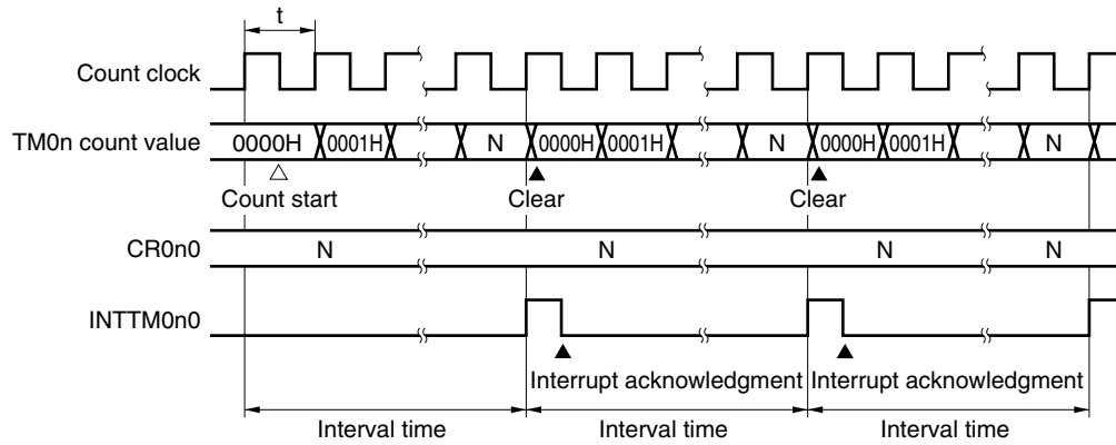
Figure 7-4. Timing of Interval Timer Operation
