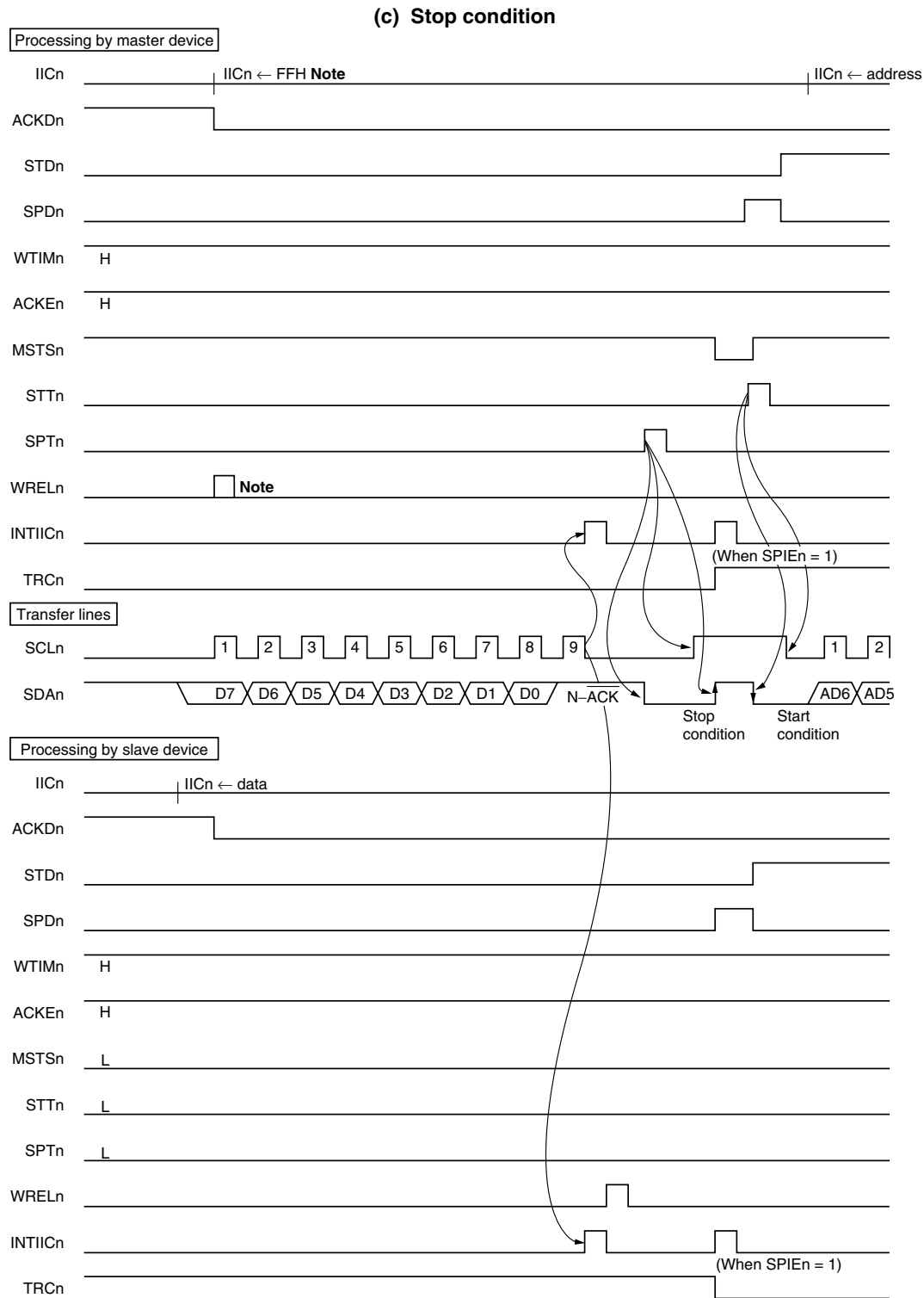
Figure 18-20. Example of Slave to Master Communication (When 9-Clock Wait Is Selected for Both Master and Slave) (3/3)
