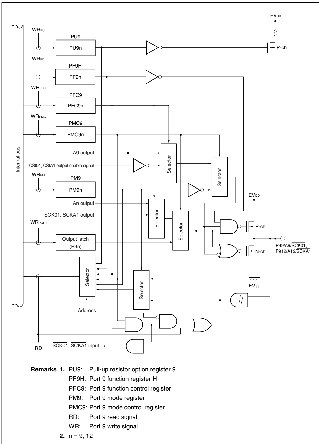
Figure 4-29. Block Diagram of P99 and P912
