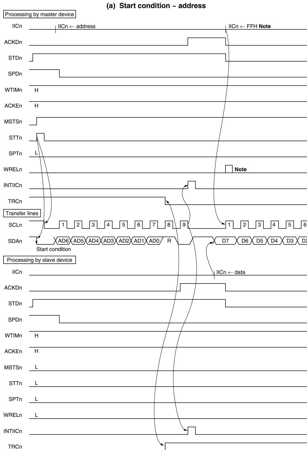
Figure 18-20. Example of Slave to Master Communication (When 9-Clock Wait Is Selected for Both Master and Slave) (1/3)
