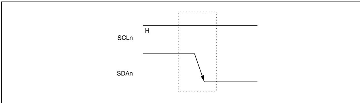
Figure 18-6. Start Conditions
