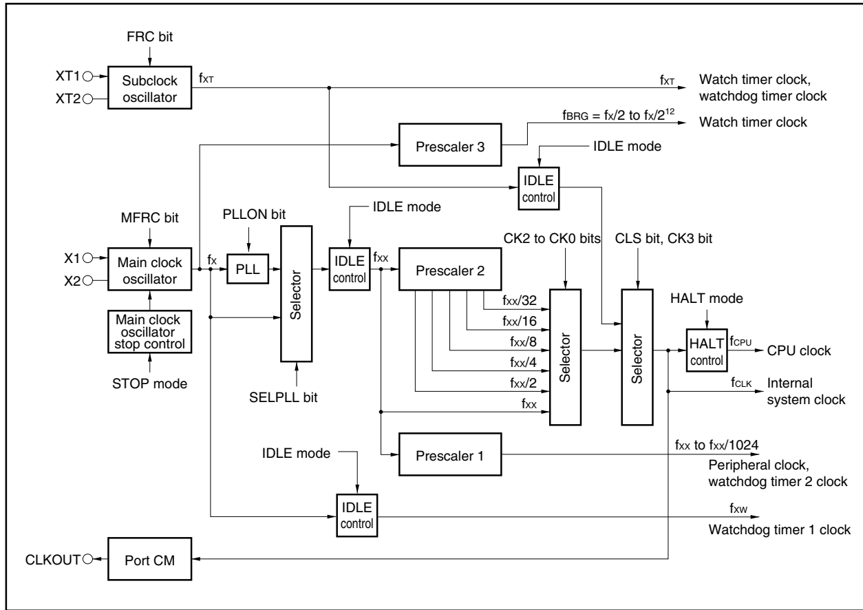
Figure 6-1. Clock Generator
