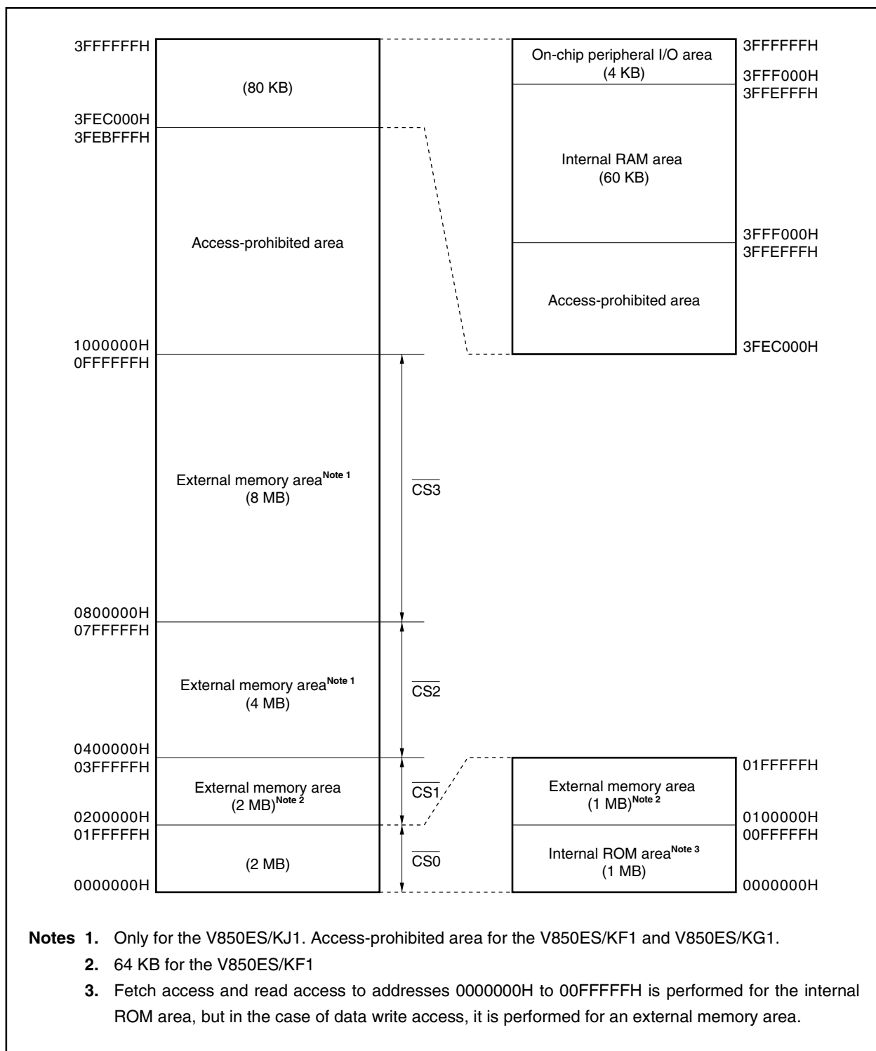
Figure 3-3. Data Memory Map (Physical Addresses)
