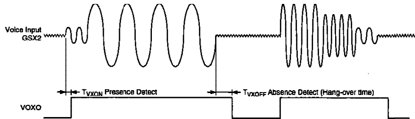
Figure 6. Transmit VOX Function
