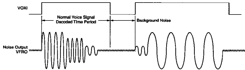
Figure 7. Receive VOX Function (CR6/B3 = 0)
