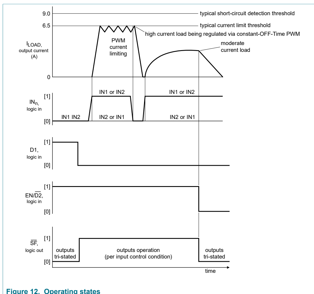
Figure 12. Operating states
