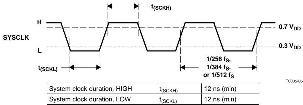
Figure 34. System Clock Timing
