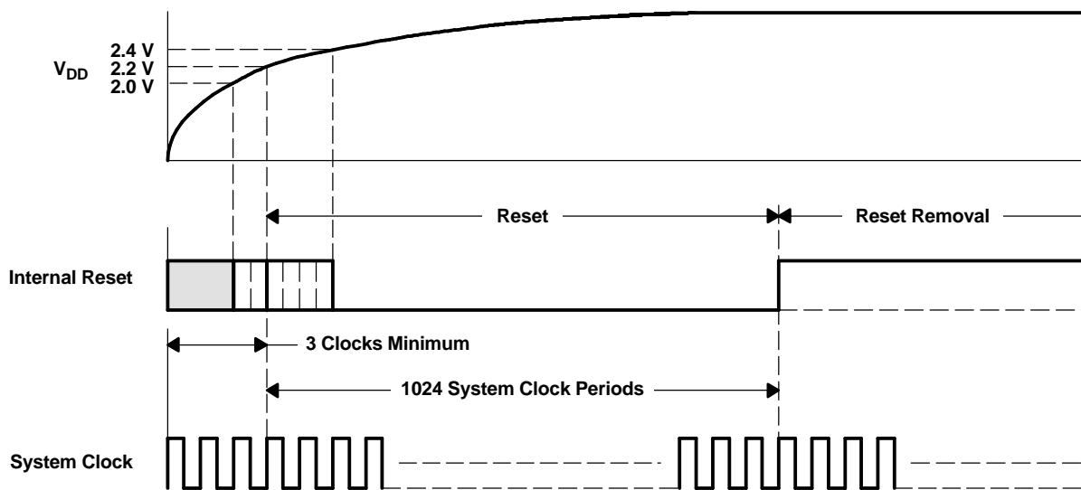
Figure 35. Internal Power-On Reset Timing
