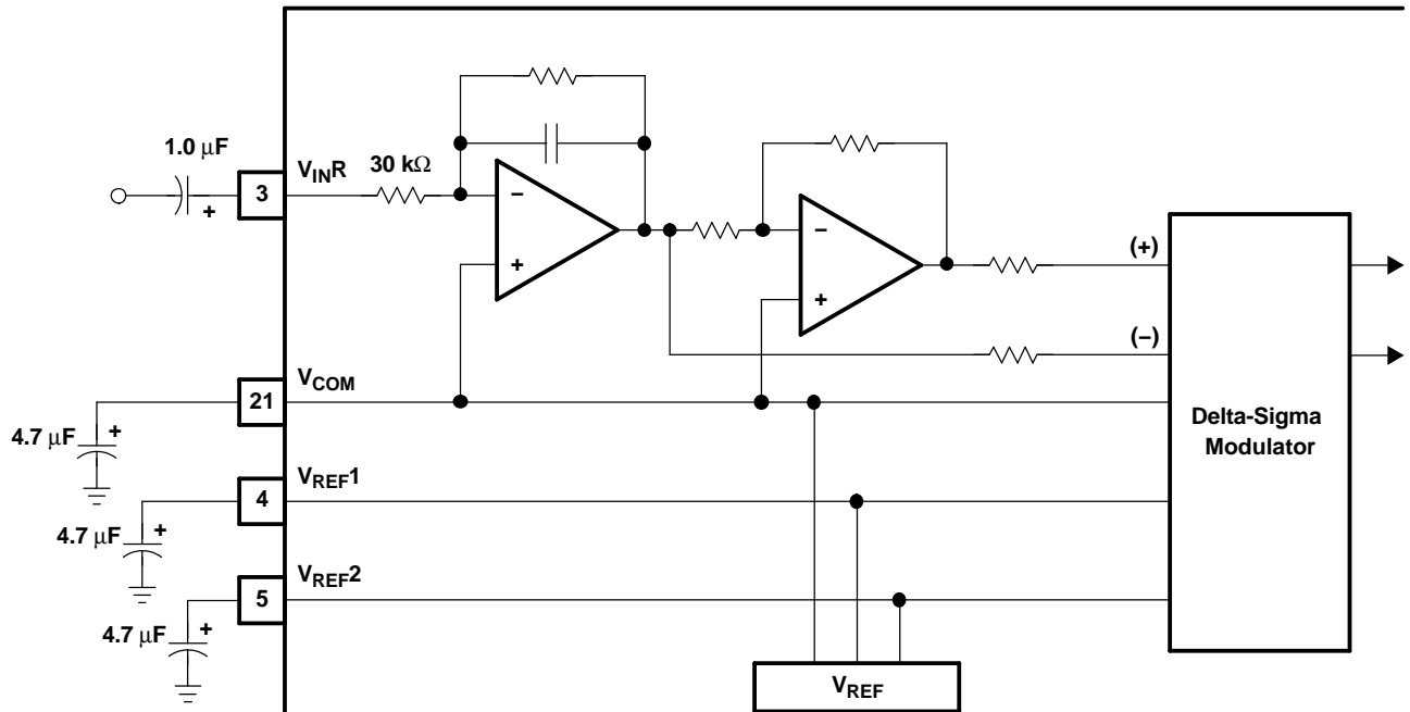
Figure 31. Analog Front End (Single-Channel)
