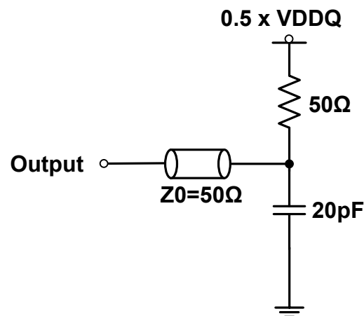
Figure 4. LVCMOS A.C. Test Load
