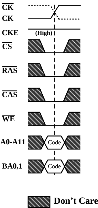
Figure 8. Mode Register Set Command
