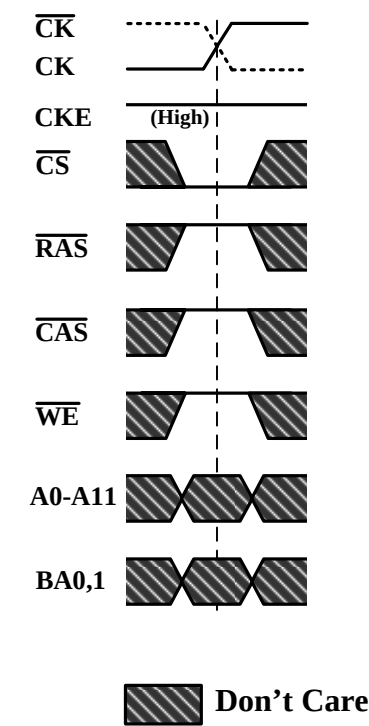
Figure 7. NOP Command
