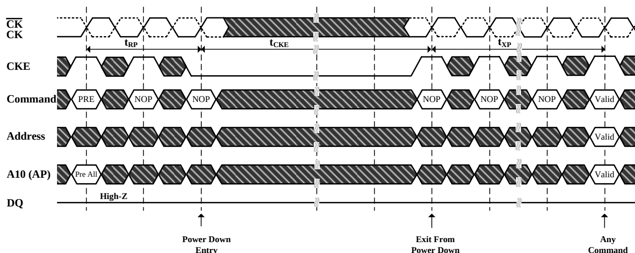
Figure 37. Power-Down Entry and Exit
