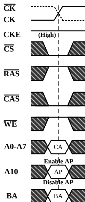
Figure 12. Read Command
