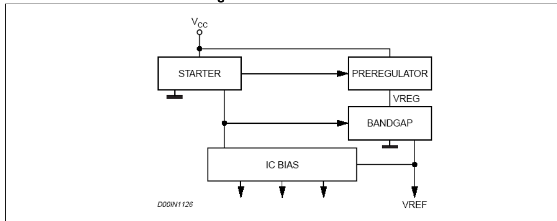
Figure 3. Internal circuit
