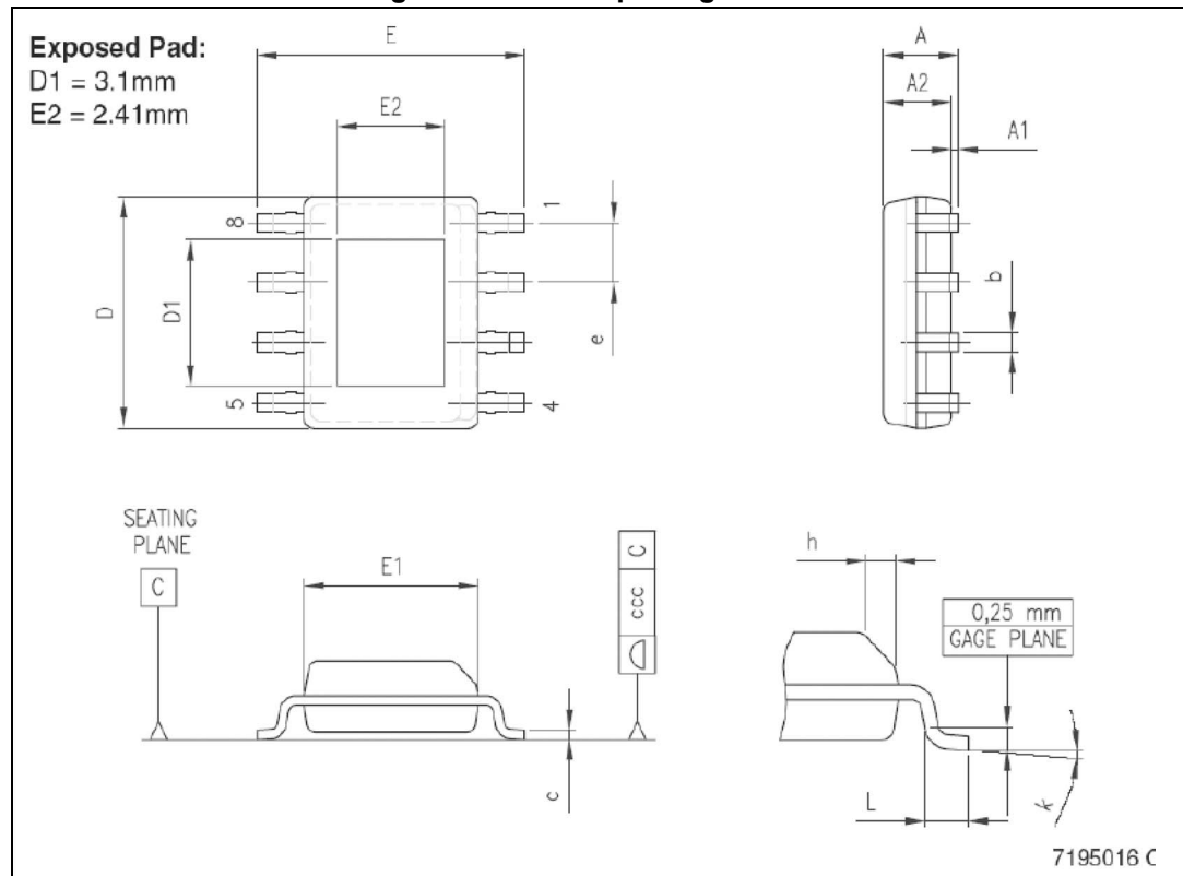
Figure 31. HSOP8 package outline
