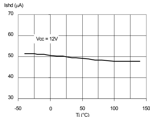
Figure 28. Shutdown current vs. junction temperature
