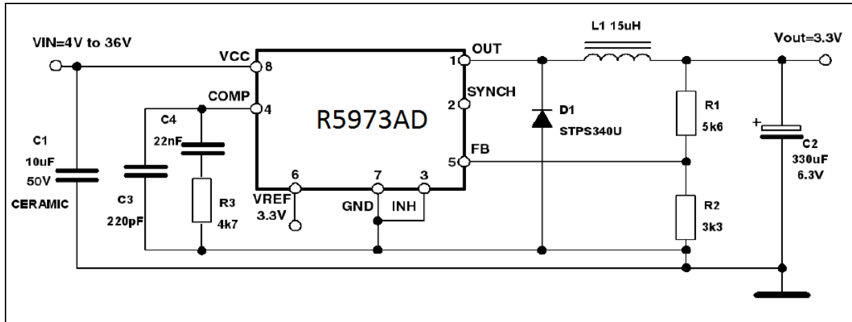
Figure 12. Application schematic
