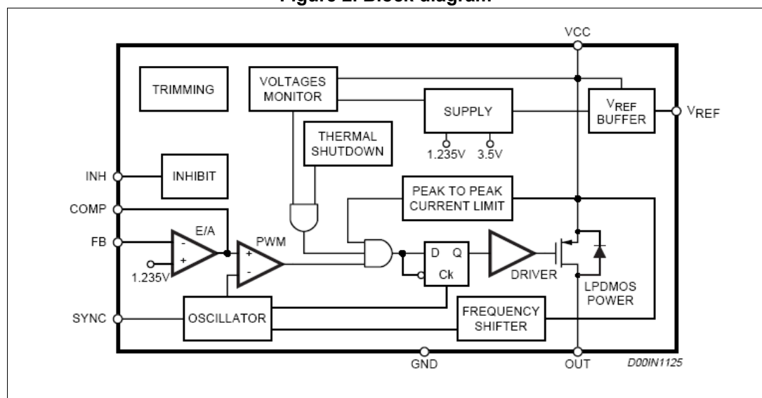
Figure 2. Block diagram
