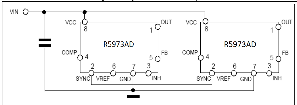
Figure 20. Synchronization example
