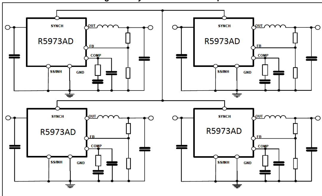
Figure 5. Synchronization example
