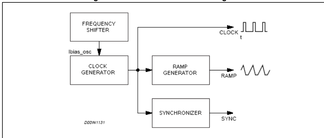
Figure 4. Oscillator circuit block diagram
