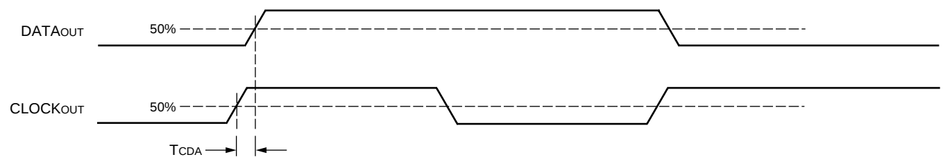
Figure 4. Clock/Data Alignment
