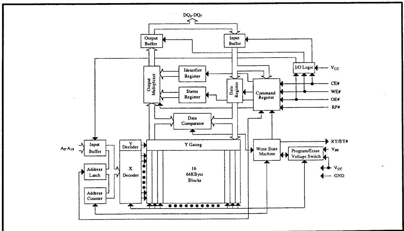
Figure 1. Block Diagram
