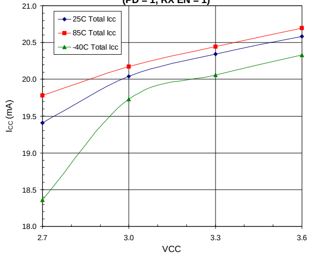
Total I_{CC} versus VCC (PD = 1, RX EN = 1)
