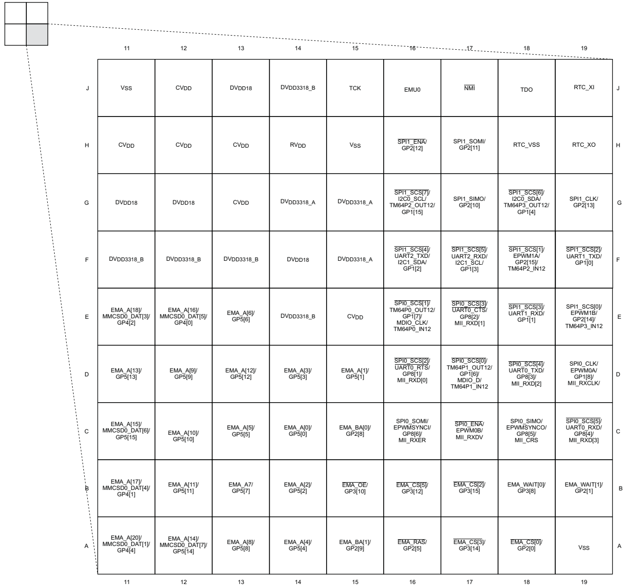
Figure 3-5. Pin Map (Quad C)
