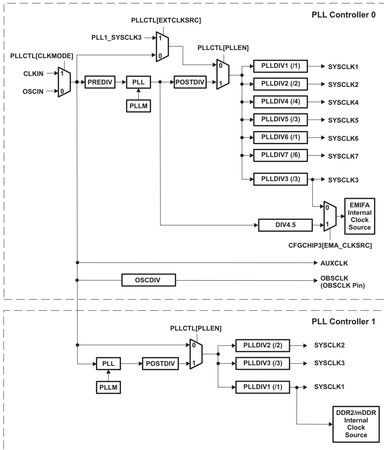
Figure 6-9. PLL Topology
