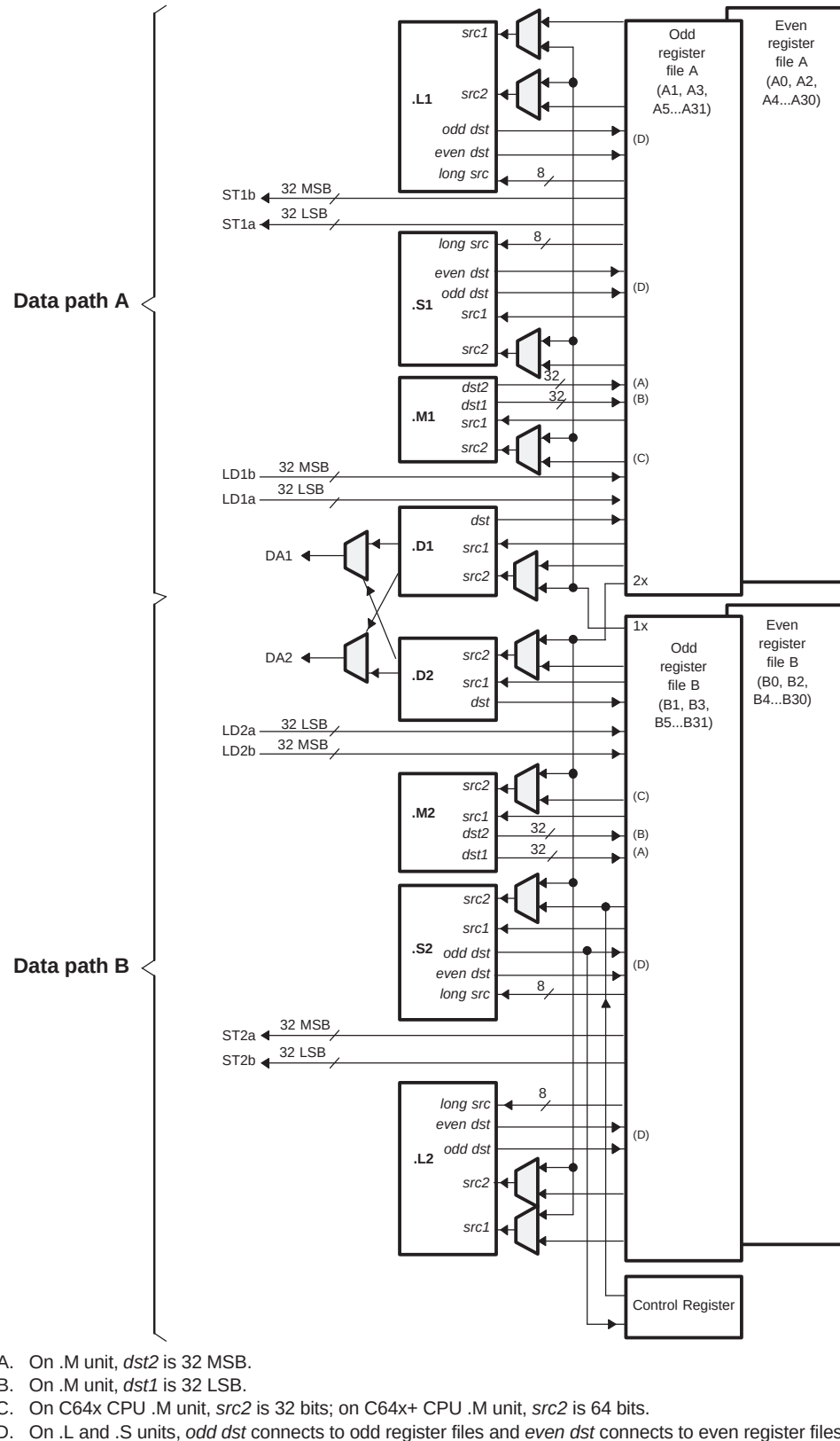
Figure 3-2. TMS320C674x CPU (DSP Core) Data Paths
