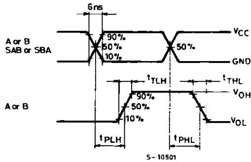
WAVEFORM 1
