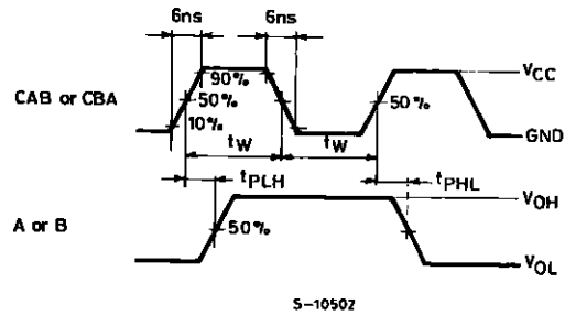
WAVEFORM 2
