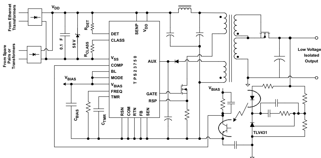
Figure 1. Typical Application
