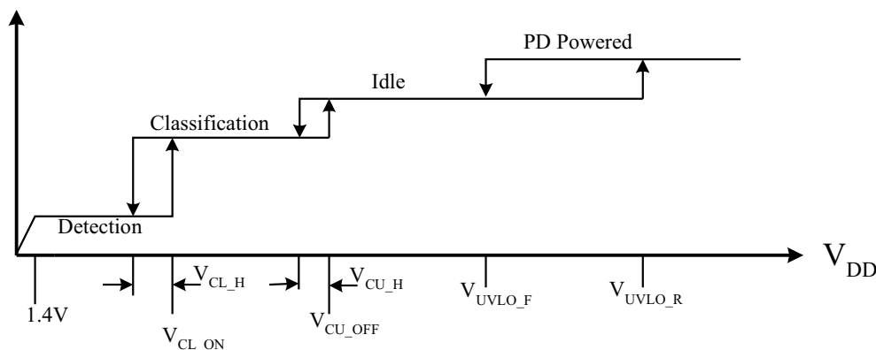
Figure 30. Threshold Voltages
