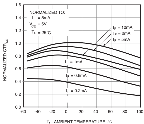
Figure 3. Normalized CTR vs. Temperature
